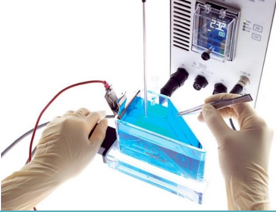
BANYO ORGANİK ANALİZLERİ (HULL-CELL)
